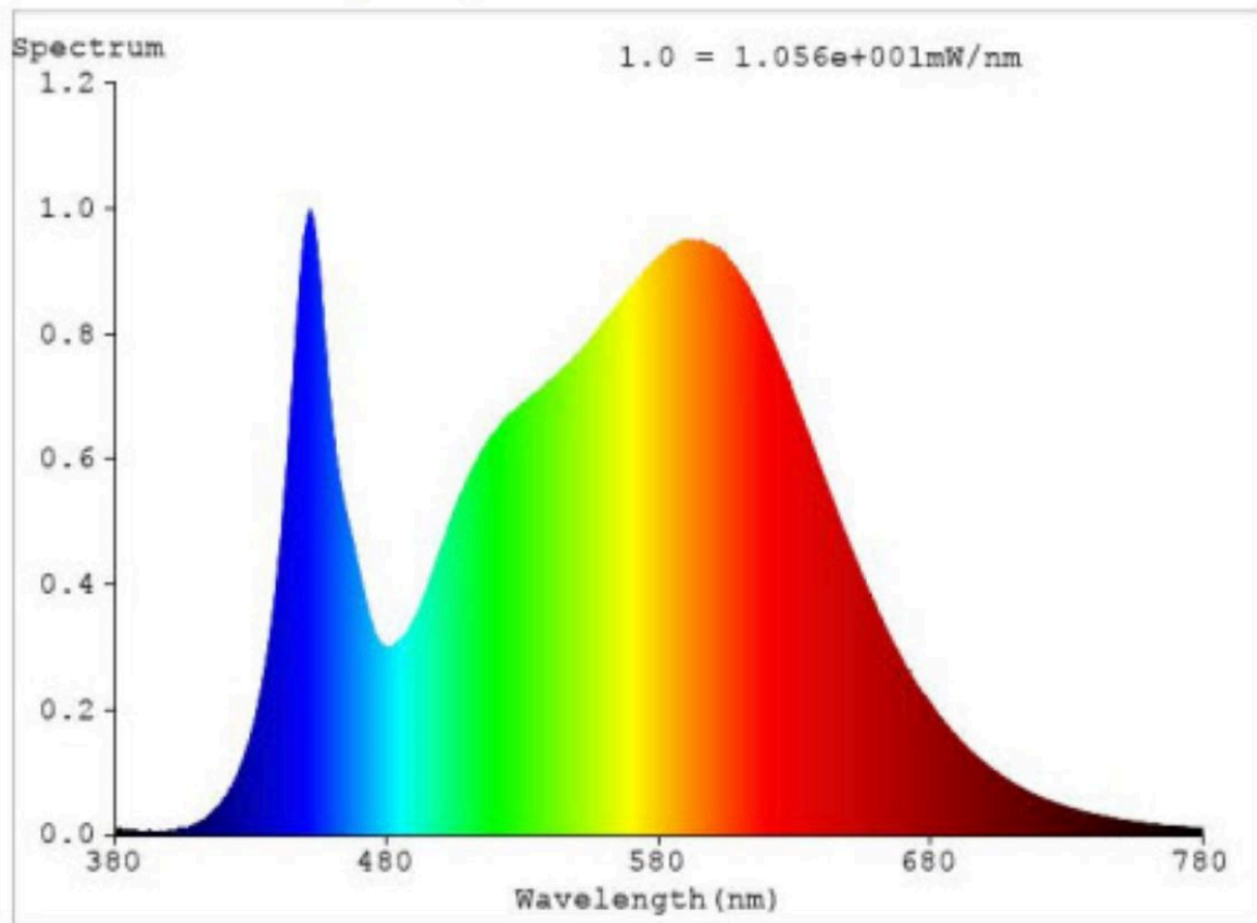
Spectral power distribution for 4000K
