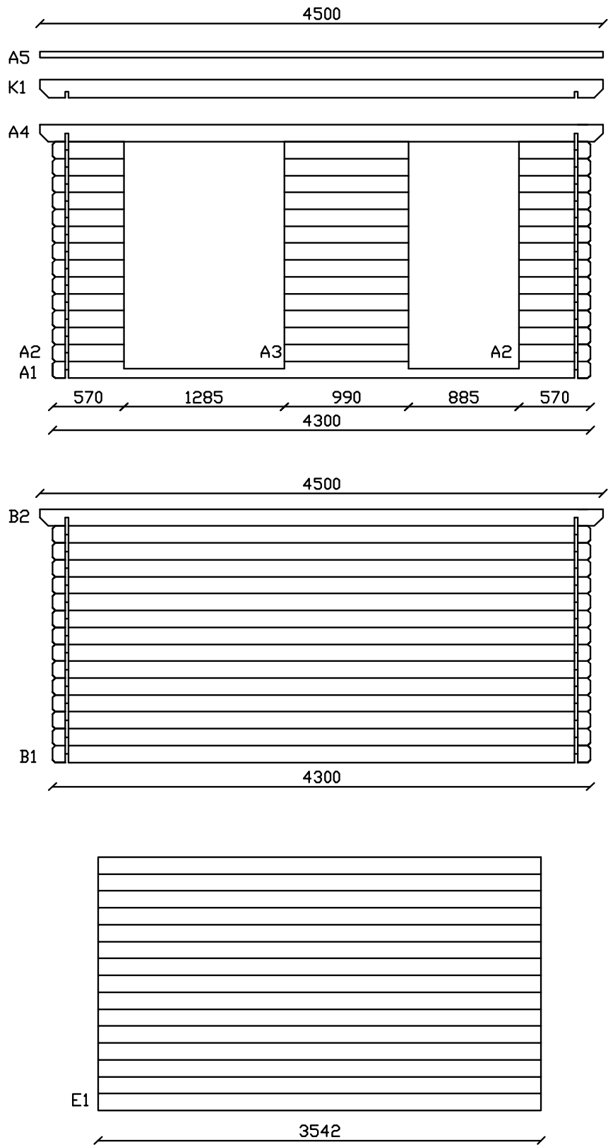
Lillevilla 59-2: 4100 x 3600 mm
